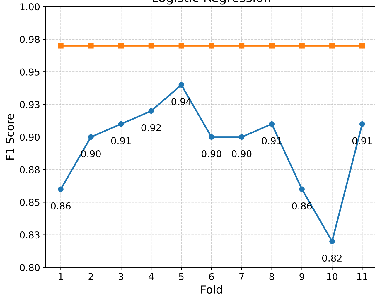
Logistic Regression
