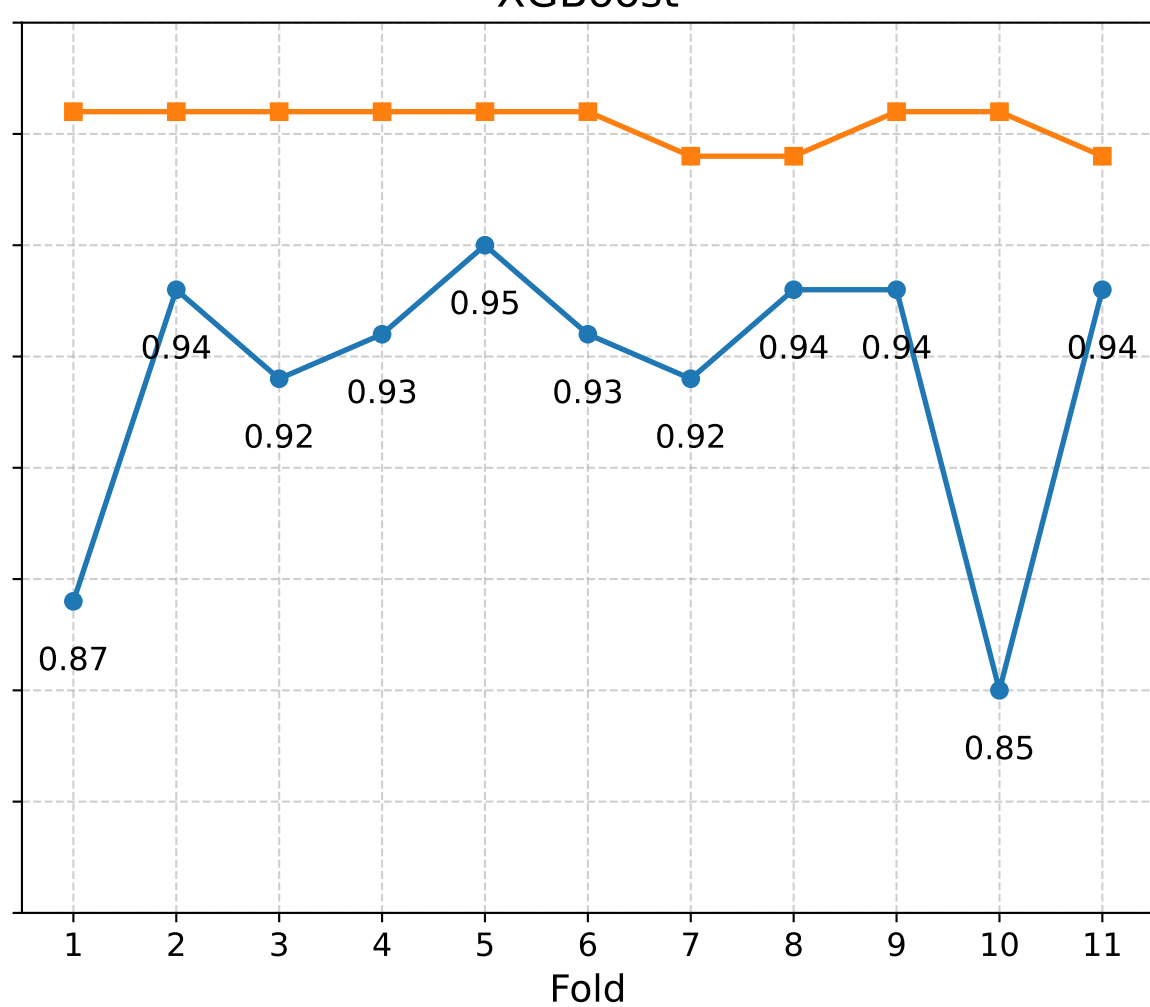
XGBoost
